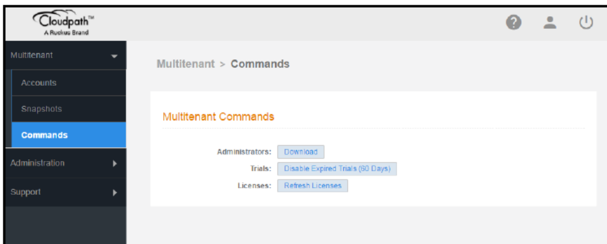
FIGURE 15 Commands View
