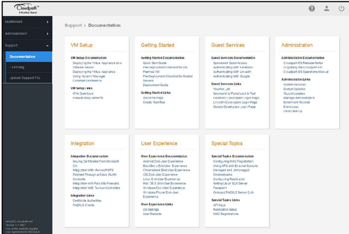
FIGURE 21 Documentation View
