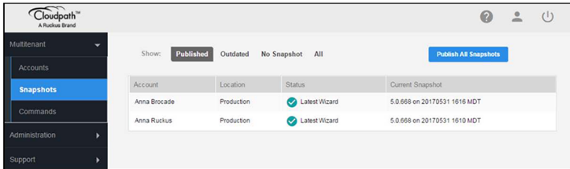
FIGURE 14 Snapshots View
